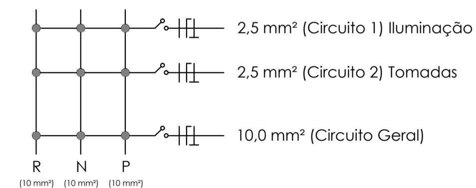
DIAGRAMA UNIFILAR PVTO SUPERIOR
